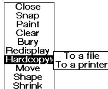
Figure 7-13. Hardcopy Submenu
