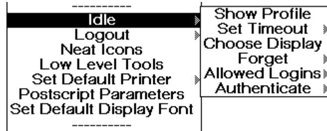
Figure 7-28. Idle Submenu
