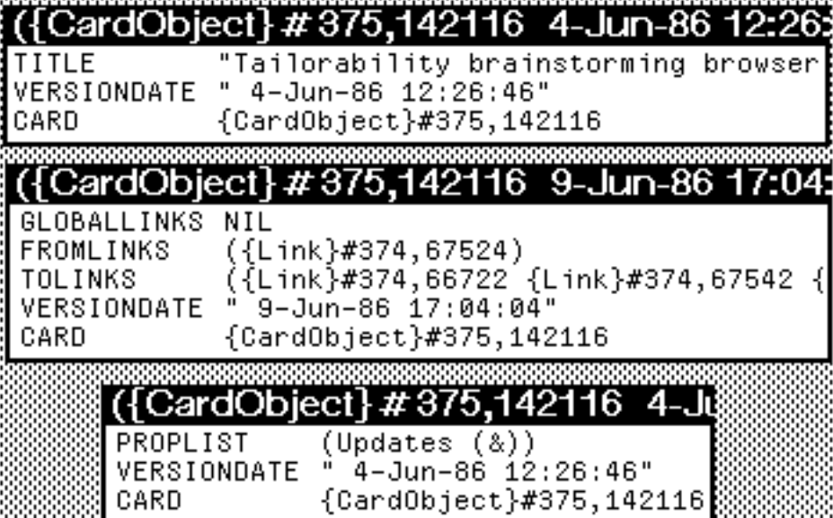
Figure B-7: Card part version inspectors for title, links and prop list.
